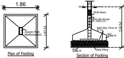
FOUNDATION DETAILS
