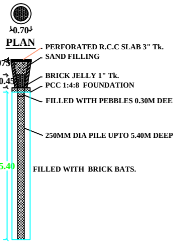
PERCOLATION PIT SECTION OF RAIN WATER
