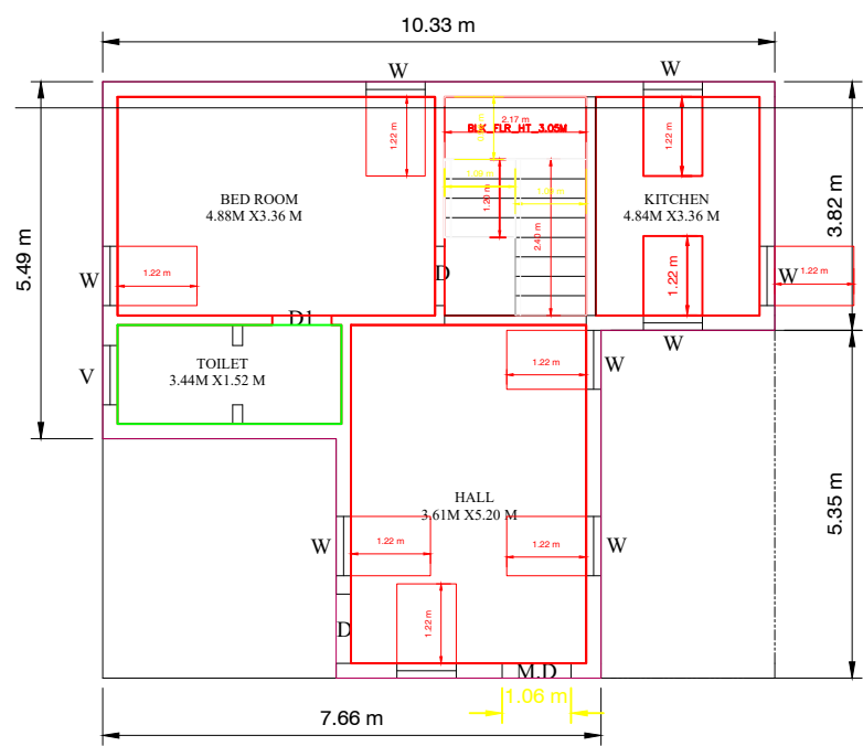
GROUND FLOOR PLAN [EAST FACING]
