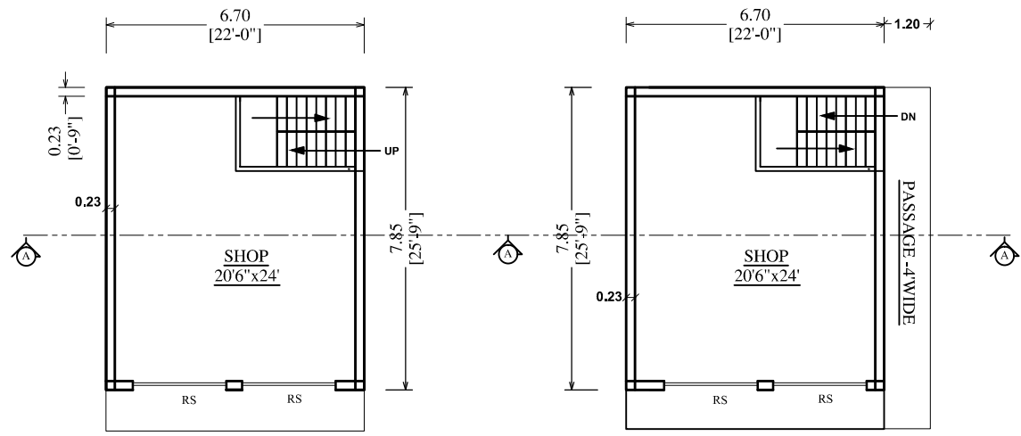
GROUND FLOOR PLAN FACED TO WEST
