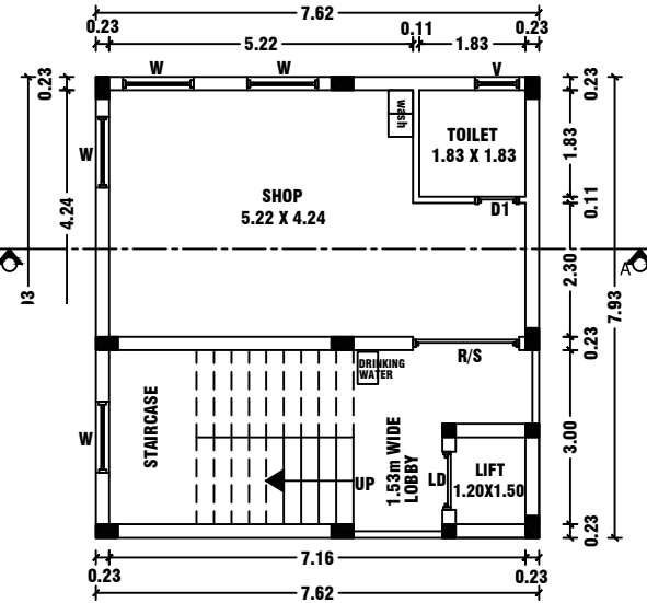
TYPICAL FIRST & SECOND FLOOR PLAN
