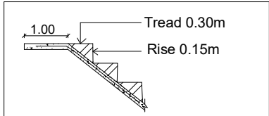
STAIRCASE DETAILS
