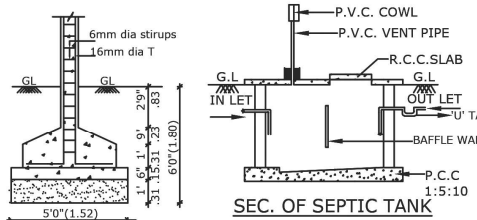
SEC. OF SEPTIC TANK
