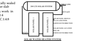
SOLAR WATER HEATER SYSTEM
