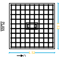
COLOUM FOUNDATION DETAILS
