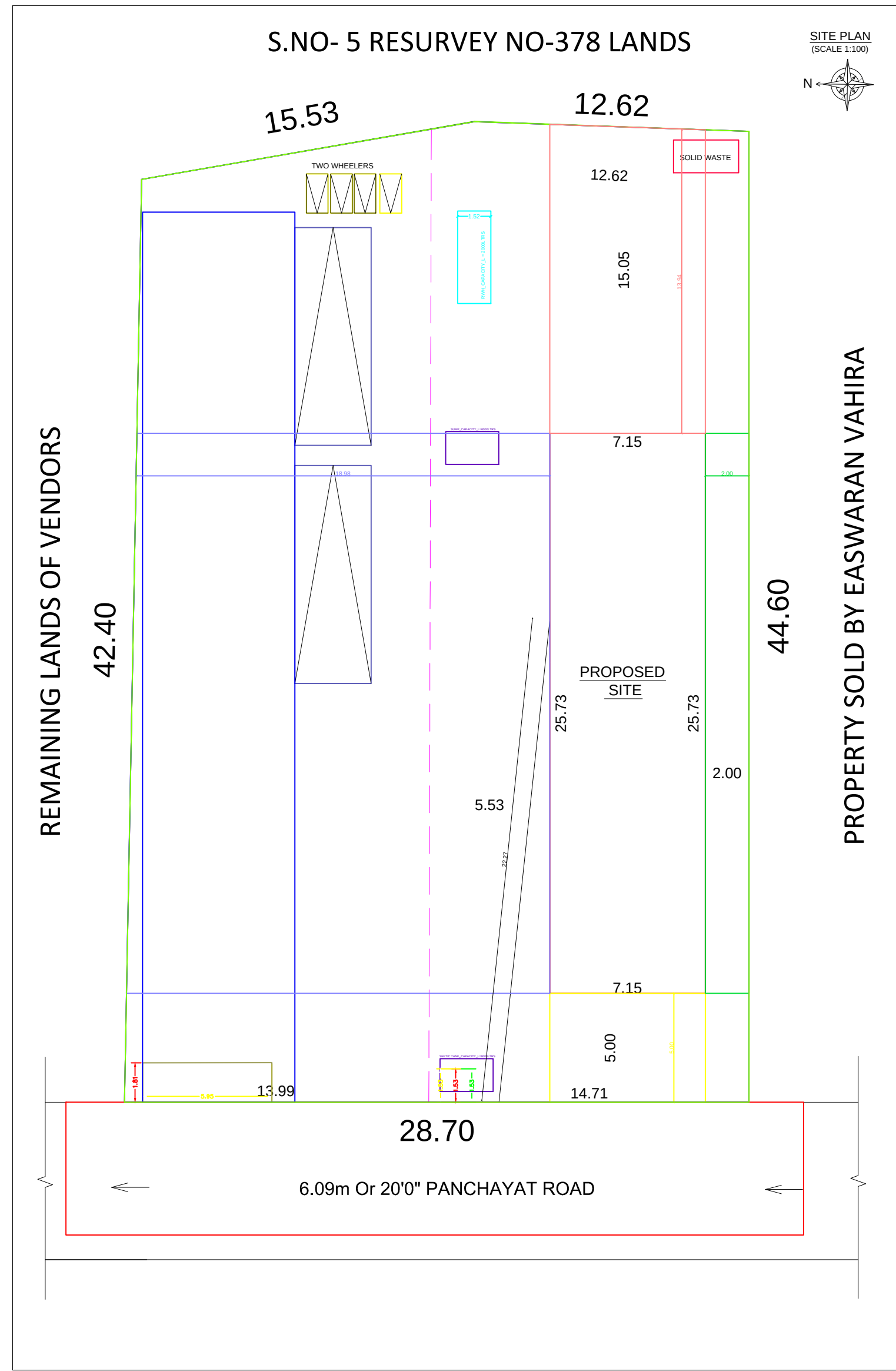
TOPO PLAN NOT TO SCALE:
