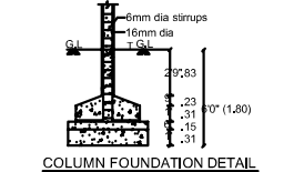
COLUMN FOUNDATION DETAIL
