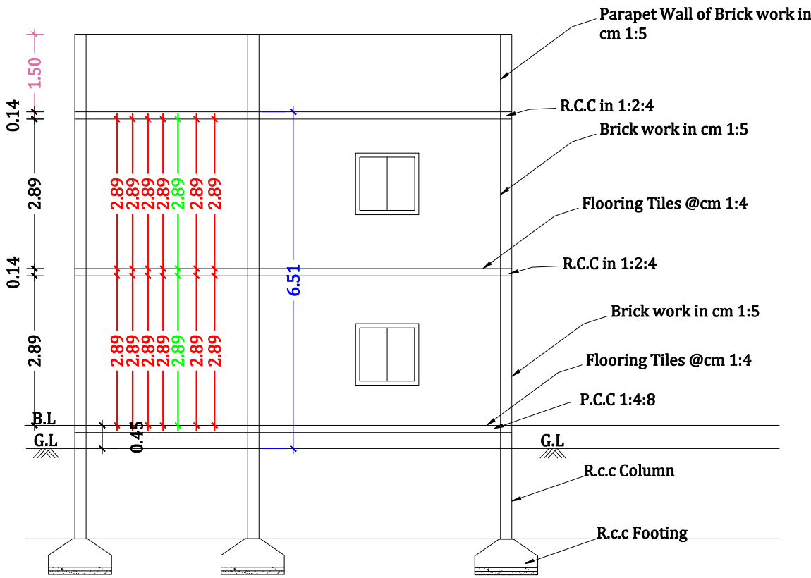
SECTION IN AA SCALE 1:100
