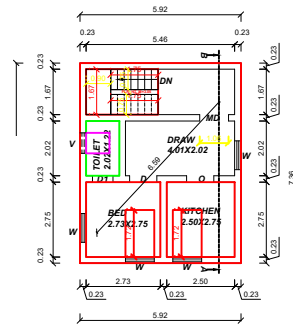
PROPOSED SECOND FLOOR PLAN
