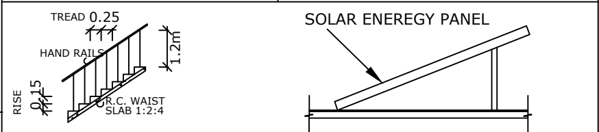
STAIRCASE DETAILS
