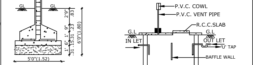
COLUMN FOUNDATION DETAIL
