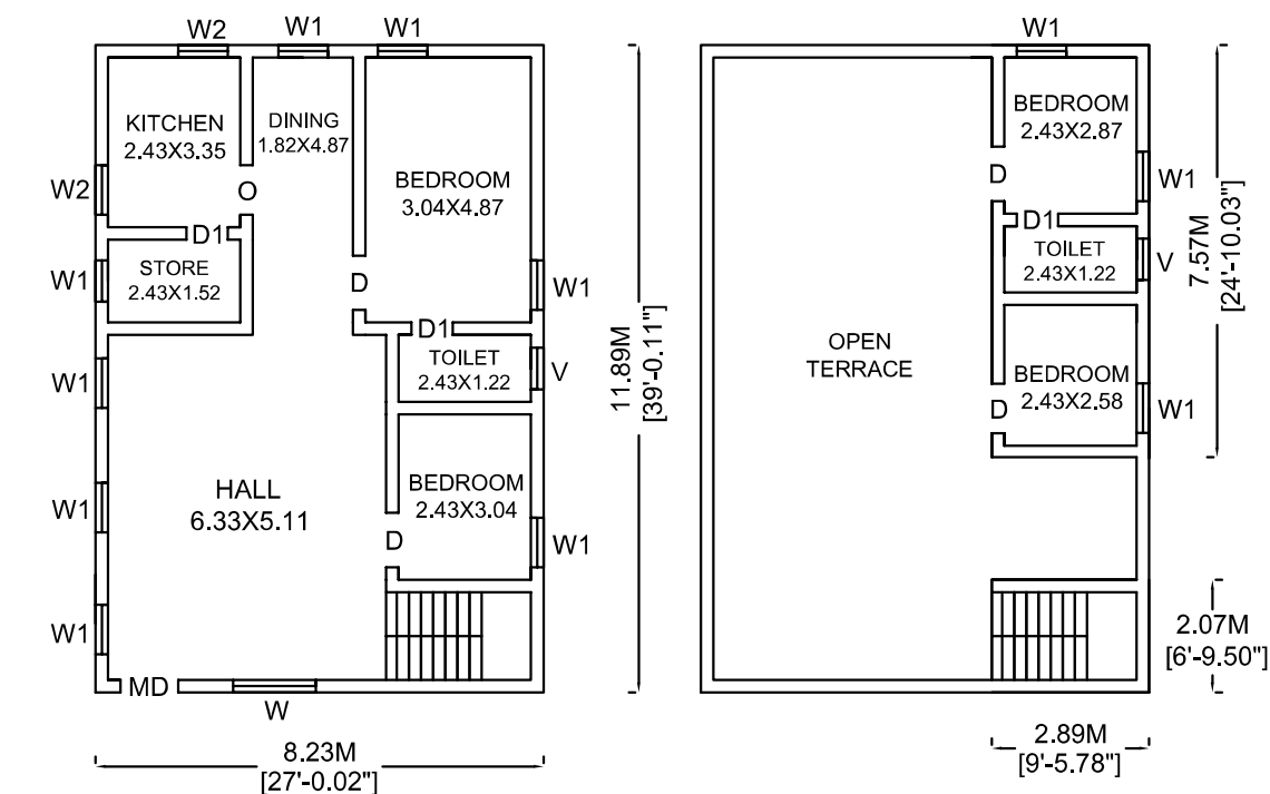
PRO. FIRST FLOOR PLAN
