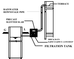
RAIN WATER COLLECTION TANK COLLECTION OF RAIN WATER FROM BUILDING
