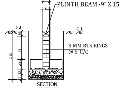
COLUMN & FOOTING DETAIL
