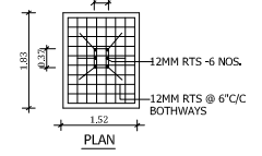
DETAILS OF SEPTICK TANK
