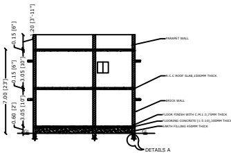
ELEVATION ON A-A
