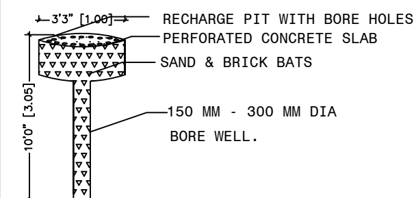
RAIN WATER HARVESTING:
