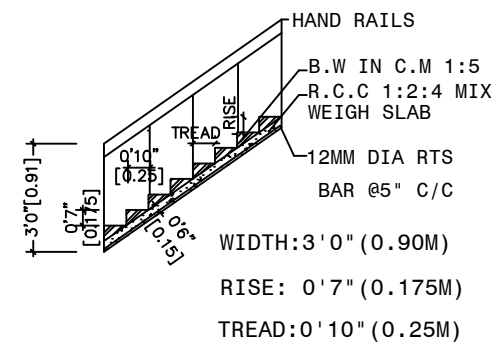
TAIR CASE DETAILS:
