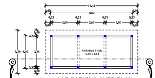
CAR PARKING SHED PLAN BLOCK - 03
