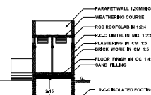
SECTION ON CC BLOCK - 02
