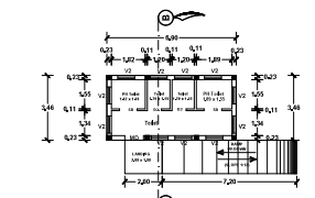
GROUND FLOOR PLAN BLOCK - 02 (Toilet Block)
