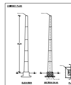
CHIMNEY PLAN
