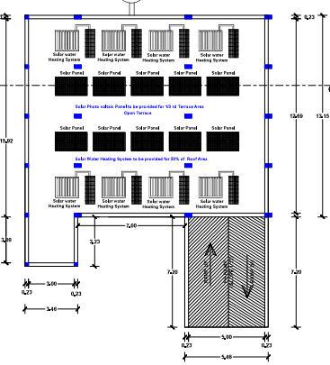
TERRACE FLOOR PLAN BLOCK - 01
