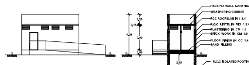
FRONT ELEVATION BLOCK - 02
