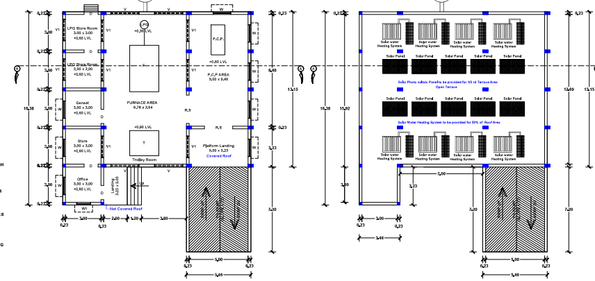
GROUND FLOOR PLAN BLOCK - 01
