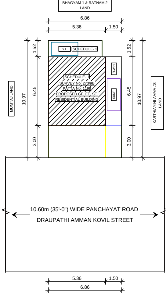
SITE PLAN
