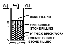
SECTION ON RAIN WATER COLLECTION TANK
