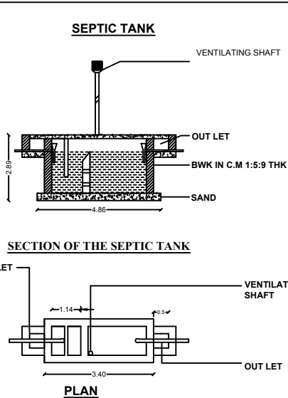
PLAN
