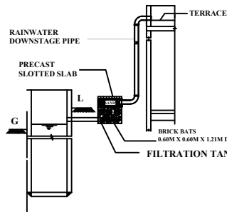
RAIN WATER COLLECTION TANK COLLECTION OF RAIN WATER FROM BUILDING
