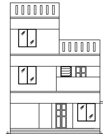
FRONT ELEVATION
