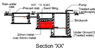
Section 'XX'
