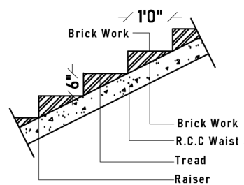
SECTION DETAIL (Not To Scale)
