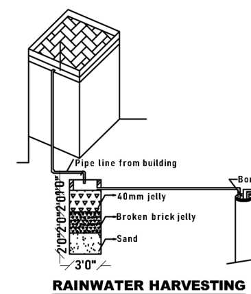
RAINWATER HARVESTING
