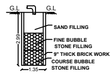
SECTION ON RAIN WATER COLLECTION TANK
