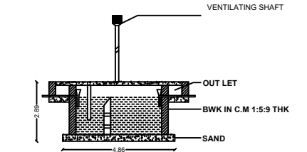
SECTION OF THE SEPTIC TANK
