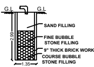
SECTION ON RAIN WATER COLLECTION TANK
