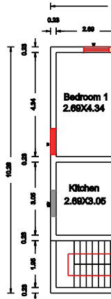
PROPOSED GROUND FLOOR PLAN
