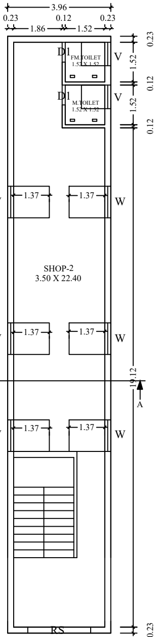
PLAN FOR FIRST FLOOR
