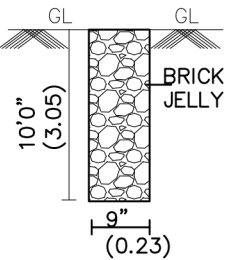
PERCULATION PIT
