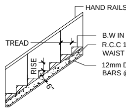
STAIRCASE DETAILS
