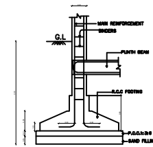
TYPICAL SECTION OF R.C.C COLUMN FOUNDATION
