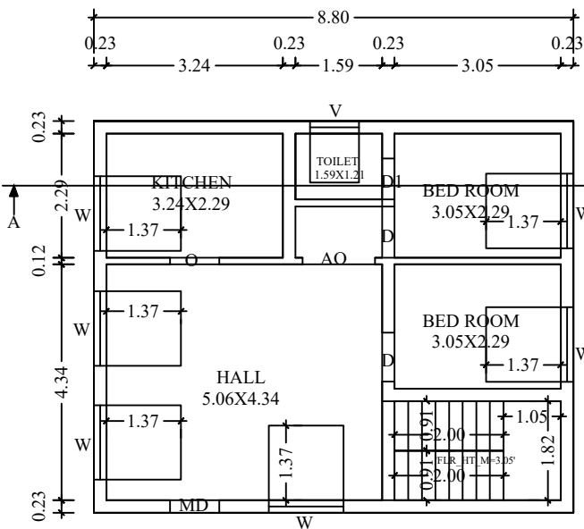
PLAN FOR GROUND FLOOR
