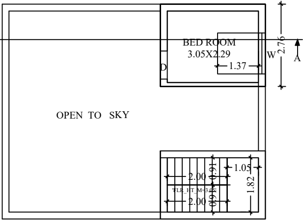
PLAN FOR FIRST FLOOR
