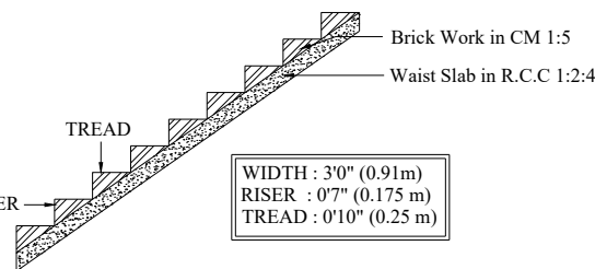
STAIRCASE DETAILS
