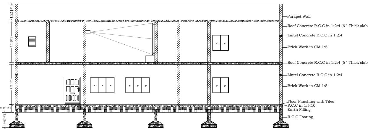
SECTION X-X
