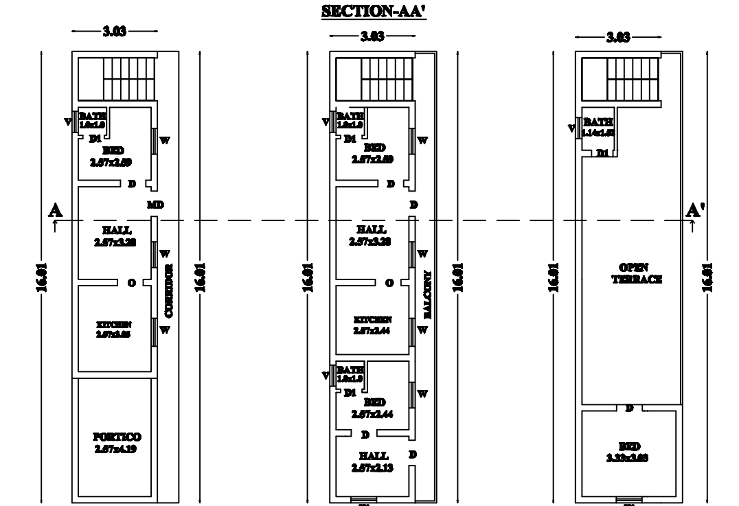
GROUND FLOOR PLAN FIRST FLOOR PLAN SECOND FLOOR PLAN
