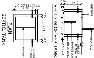
SEPTIC TANK:-
