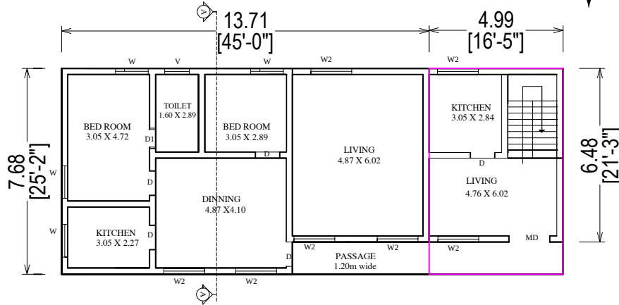
EXISTING & PROPOSED SECOND FLOOR PLAN
