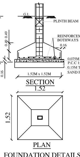
FOUNDATION DETAILS
