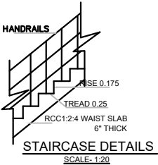
SCALE- 1:20
