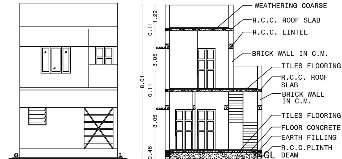
FRONT ELEVATION
