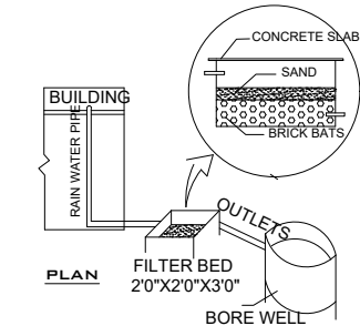
RAIN WATER HARVESTING TANK
