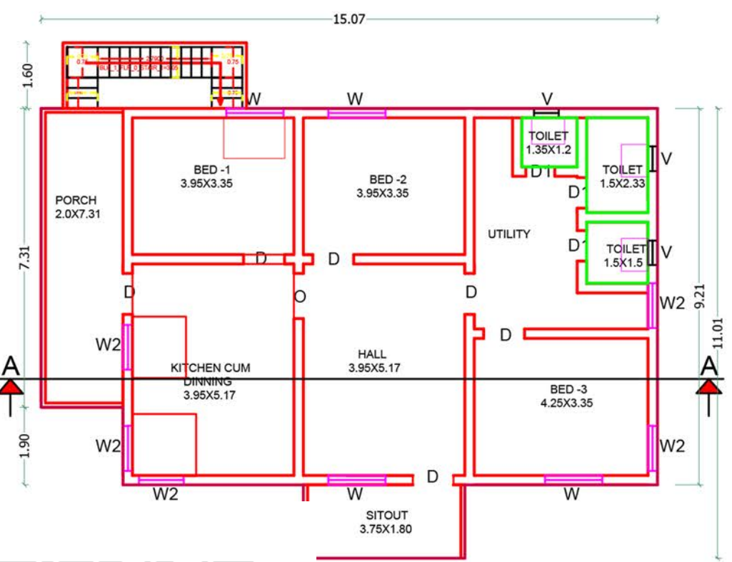
GROUND FLOOR PLAN (FACEING EAST)
