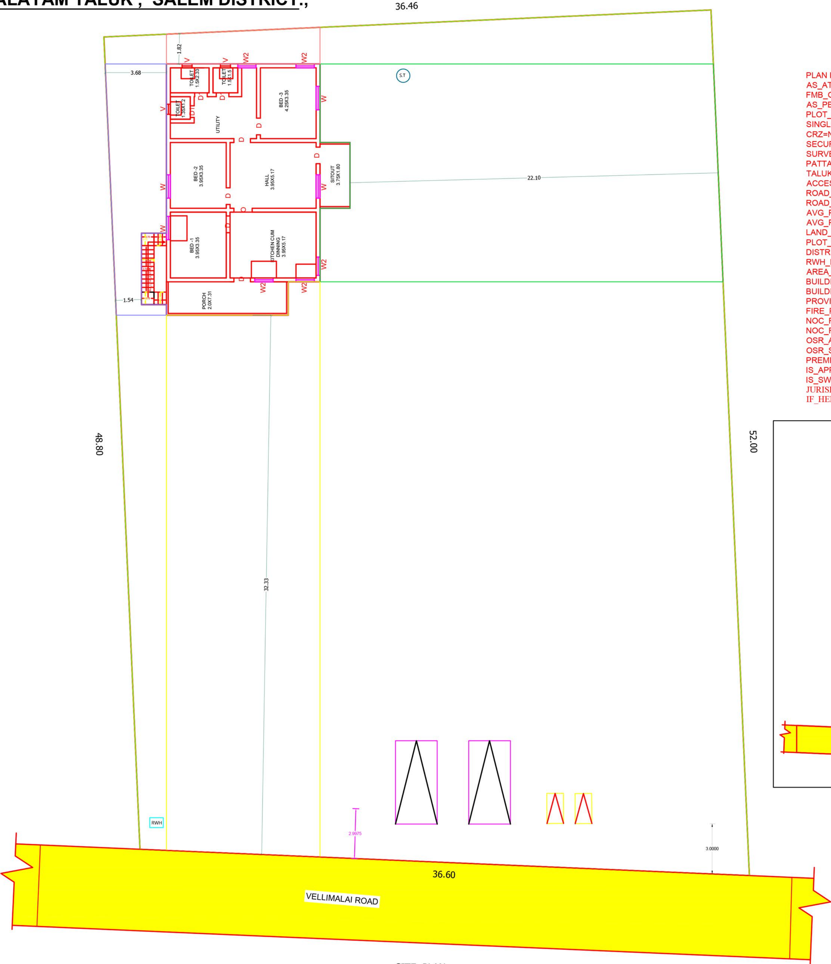
SITE PLAN
