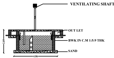
SEPTIC TANK
