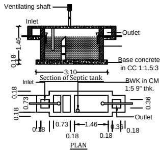
SEPTIC TANK DETAIL
