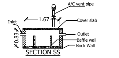
SECTION SS
