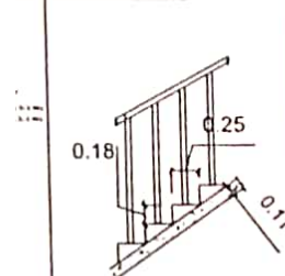
STAIRCASE DETAILS -
