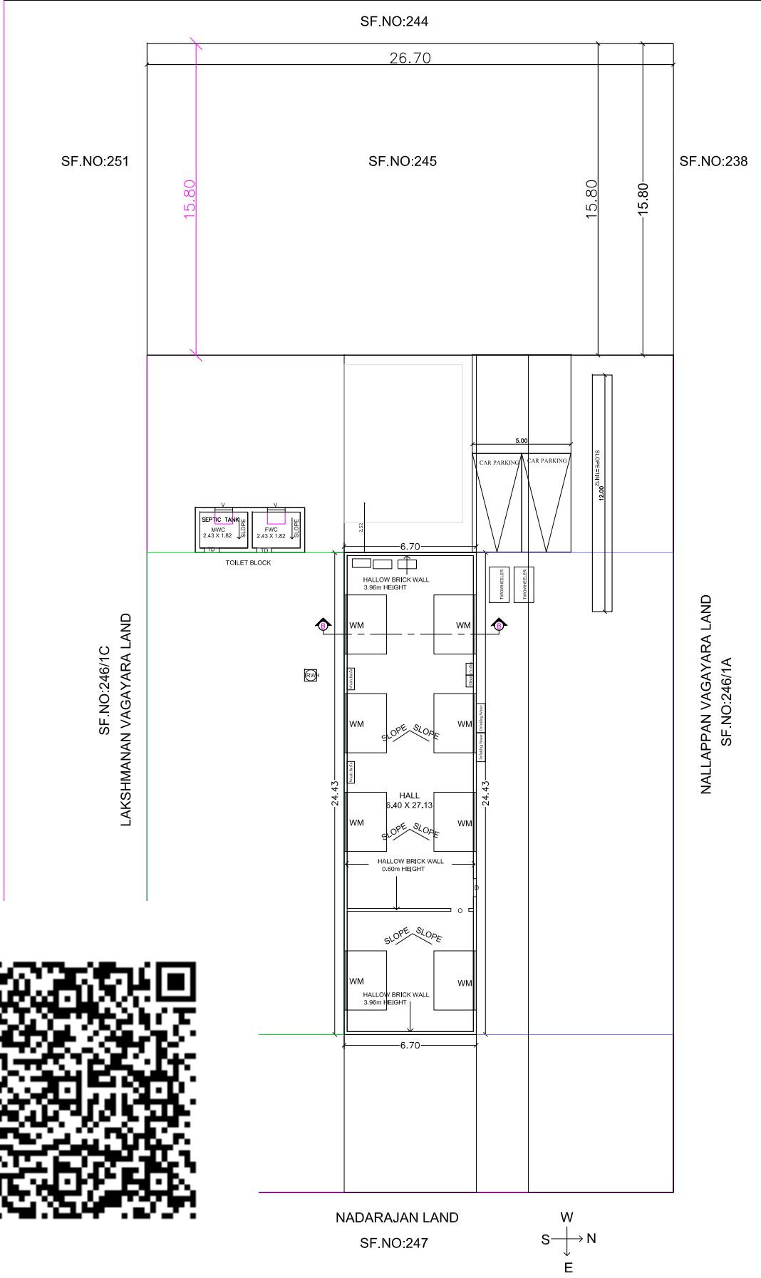
SITE CUM GROUND FLOOR PLAN
