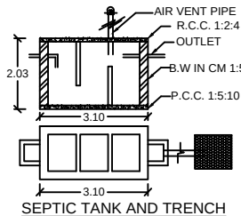
SEPTIC TANK AND TRENCH
