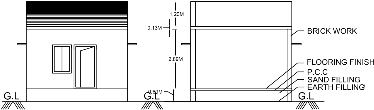
FRONT ELEVATION SECTION ON A-A
