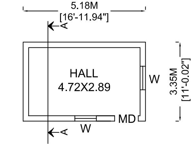
PRO.GROUND FLOORPLAN
