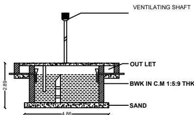
SEPTIC TANK
